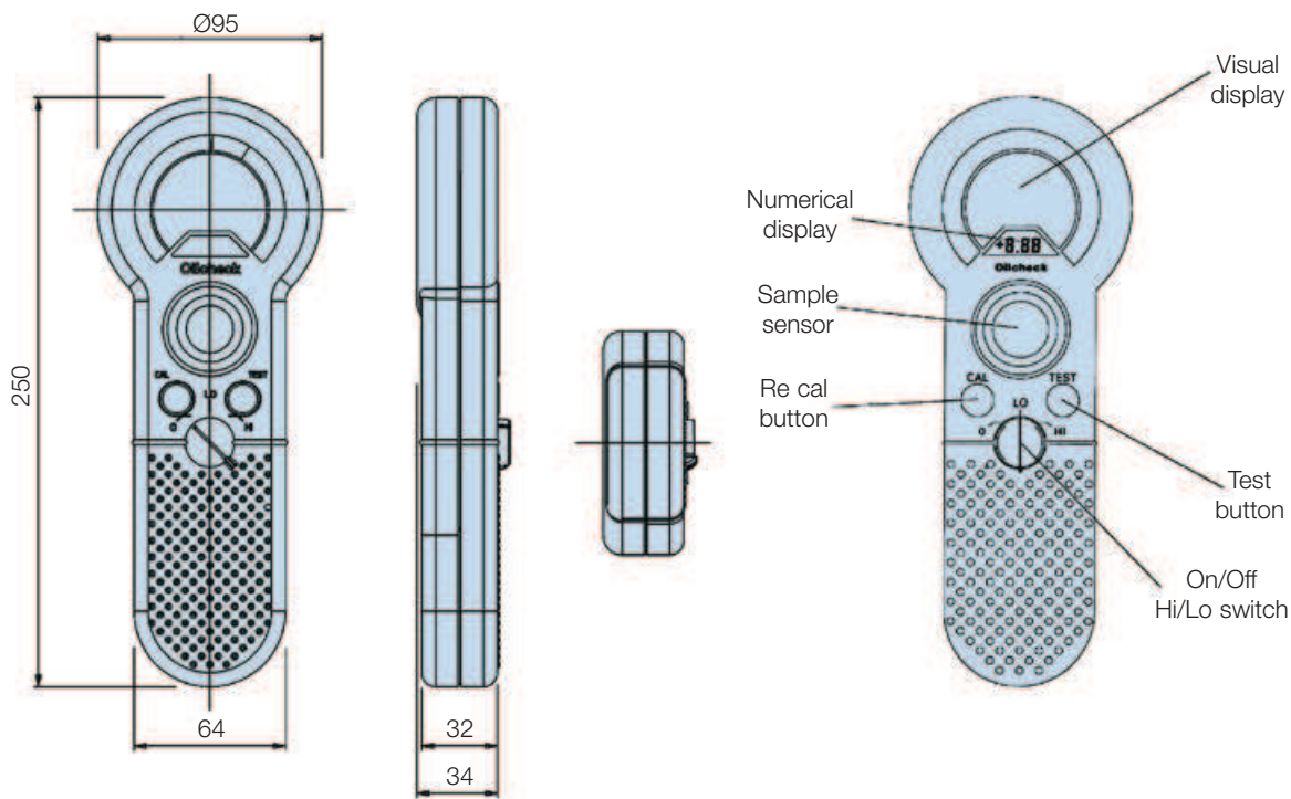
Function buttons
